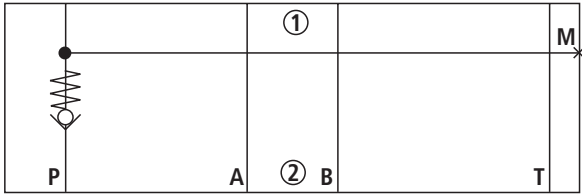
Type Z1S 6 P.-4X/... SO90
